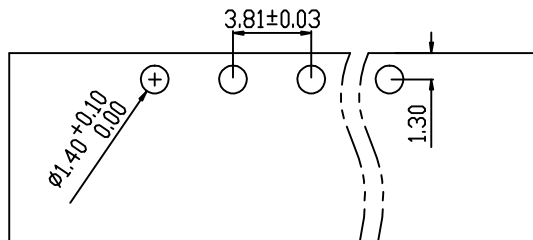
PCB LAYOUT
